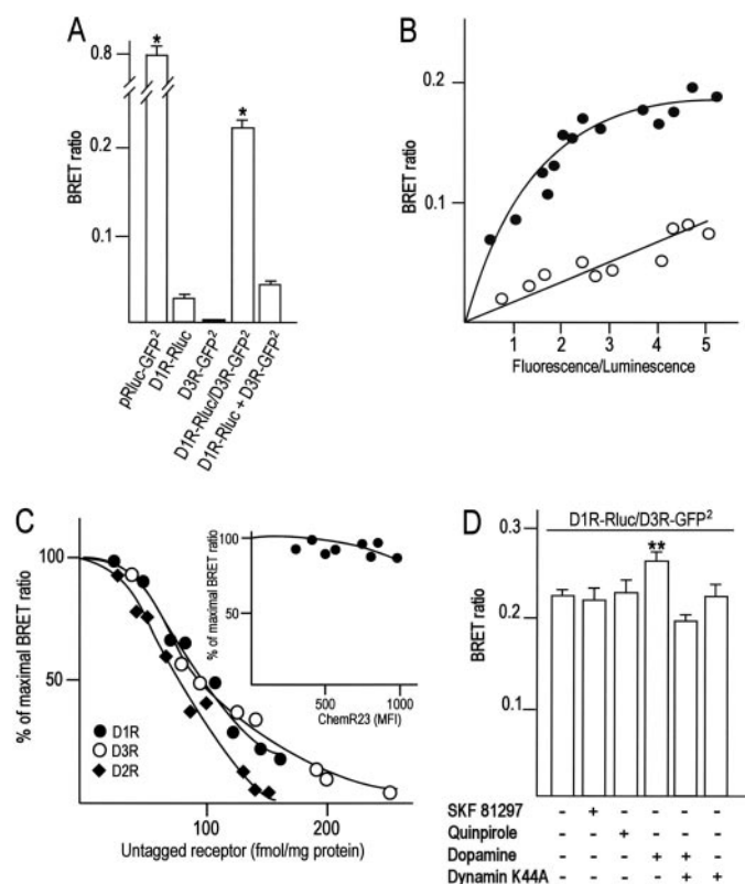
Fig. 3. Detection of D1R and D3R interaction by BRET 2 in transfected HEK 293 cells. The D1R fused to R. reniformis luciferase (D1R-Rluc) and the D3R fused to GFP 2 (D3R-GFP 2 ) were transfected either individually or simultaneously in HEK 293 cells. The DeepBlueC coelenterazine substrate was added at a final concentration of 5 \mu M. A, quantification of BRET 2 data from a series of control experiments with single receptor constructs (D1R-Rluc, D3R-GFP 2 , and pRluc-GFP 2 ) or with D1R-Rluc and D3R-GFP 2 coexpressed in the same cells (D1R-Rluc/D3R-GFP 2 ) or with cells individually expressing D1R-Rluc and D3R-GFP 2 mixed together before the BRET 2 experiment (D1R-Rluc + D3R-GFP 2 ). Bars are the means \pm S.E. of five experiments. *, p < 0.001 versus D1R-Rluc, Student's t test. B, BRET 2 titration analysis. Cells were transfected with D1R-Rluc in the presence of increasing concentrations of either D3R-GFP 2 or ChemR23-GFP 2 . BRET 2 , total luminescence, and total fluorescence were determined. BRET 2 ratio values are plotted as a function of the total fluorescence/total luminescence ratio. Data are representative of three experiments. The curves were fitted using a nonlinear regression equation assuming a single binding site (GraphPad Prism 4). ●, specific BRET 2 signal generated in the presence of D3R-GFP 2 ; ○, nonspecific signals generated in the presence of ChemR23-GFP 2 . C, BRET 2 competition analysis. Experiments were carried out at the constant D1R-Rluc/D3R-GFP 2 ratio of 3.4 \pm 0.5 in the absence or presence of increasing concentrations of either untagged D1R (●), D3R (○), or D2R (■). The expression of untagged receptors was determined by radioreceptor binding. Data are representative of three experiments. Inset, experiments were carried out at the constant D1R-Rluc/D3R-GFP 2 ratio of 3.4 \pm 0.5 in the absence or in the presence of increasing concentrations of untagged ChemR23. The expression of ChemR23 in each sample was determined by immunofluorescence and fluorescence-activated cell sorting analysis and is expressed as Medial Fluorescence Intensity (MFI). Data are representative of three experiments. D, cells transfected with D1R-Rluc and D3R-GFP 2 were exposed to either 1 \mu M SKF 81297 or 1 \mu M quinpirole or 10 \mu M dopamine in the absence or in the presence of dynamin-K44A. Bars are the means \pm S.E. of five independent experiments. *, p < 0.005 versus untreated cells, Student's t test.
